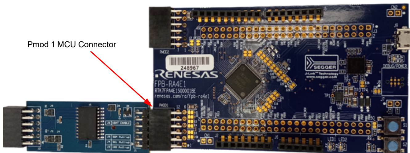
Figure 4. Evaluation Kit Connections
