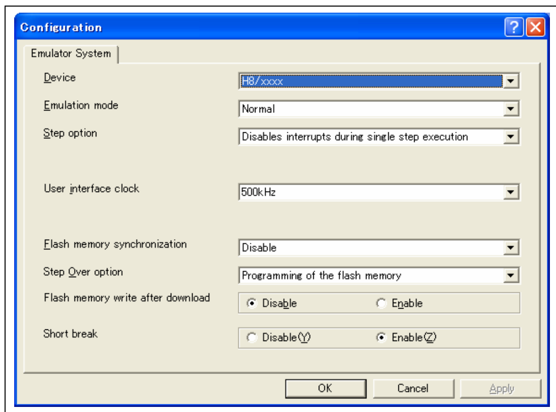
Figure 5.4 [Configuration] Dialog Box ([Emulator System] Page)
