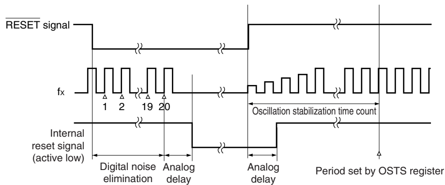
Figure 20-4. Sampling Operation Timing (20 Times)
