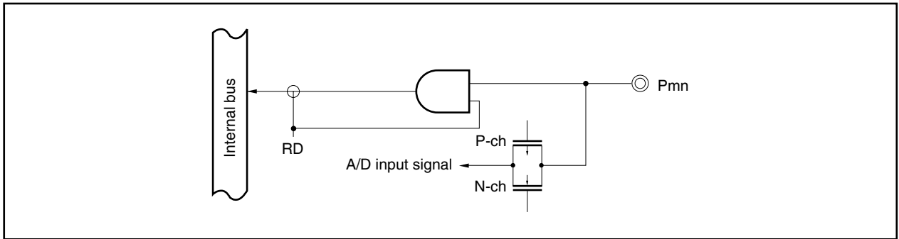
Figure 4-3. Block Diagram of Type C-U
