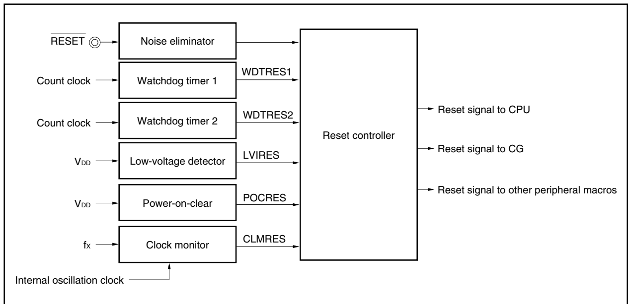
Figure 20-1. Reset Block Diagram
