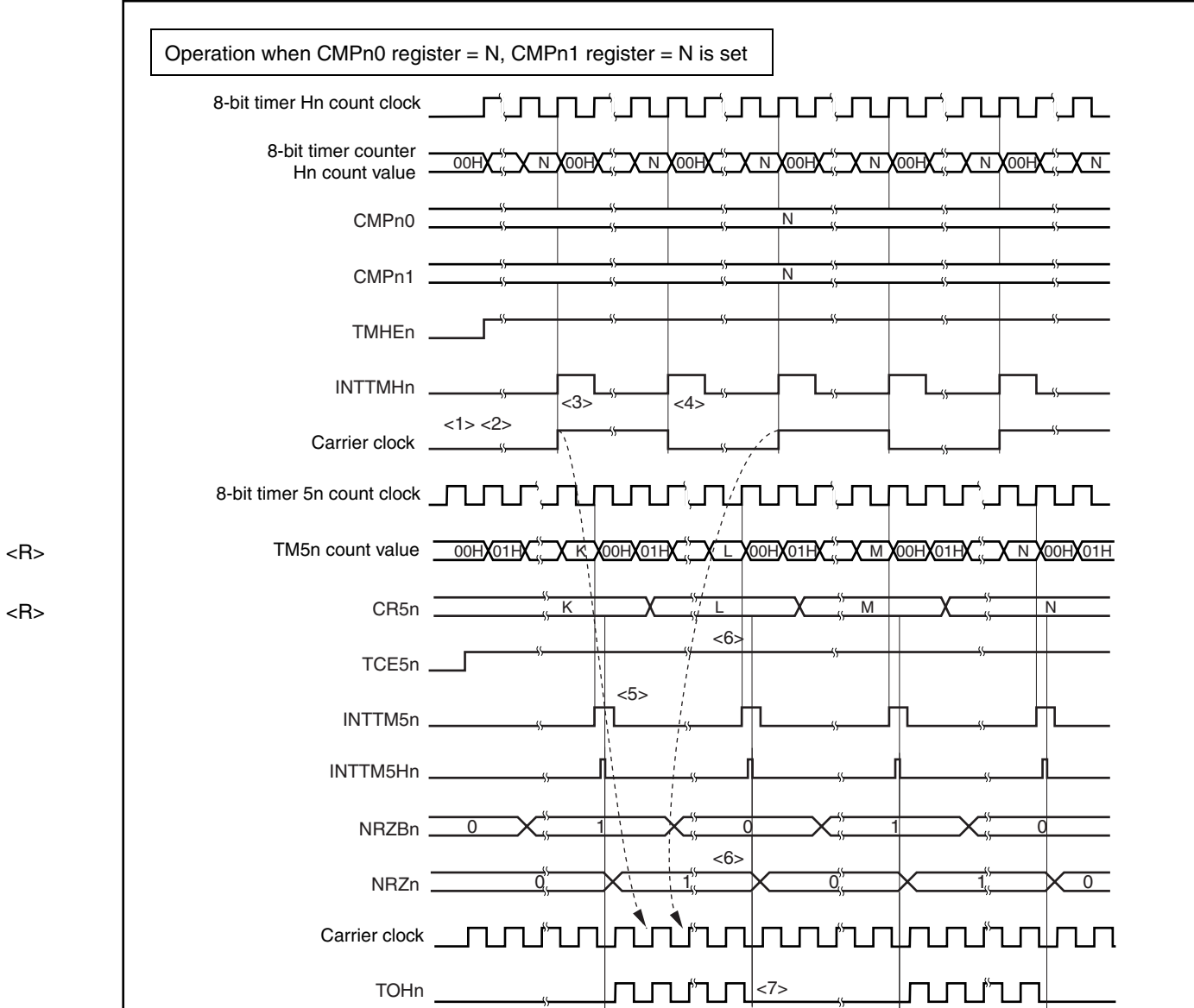
Figure 9-8. Carrier Generator Mode (1/3)
