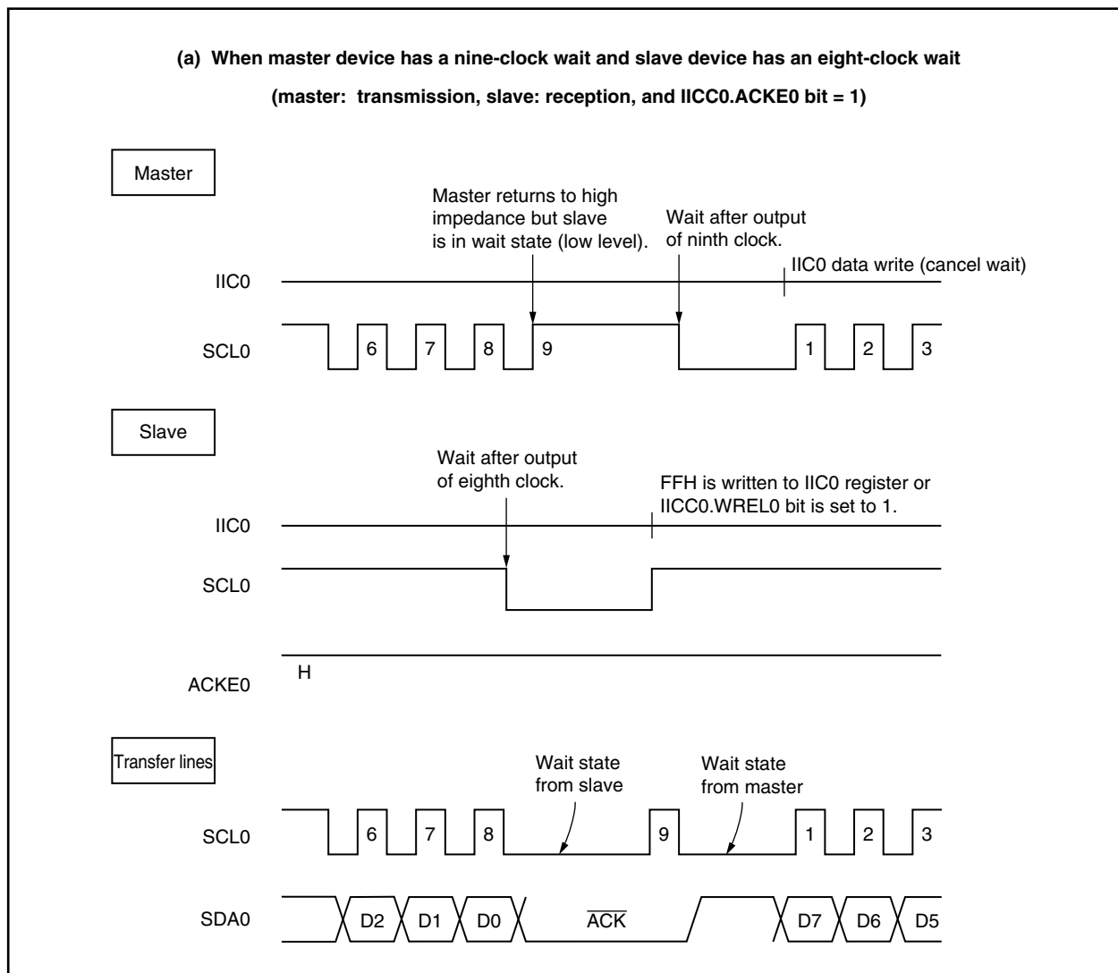
Figure 16-10. Wait State (1/2)
