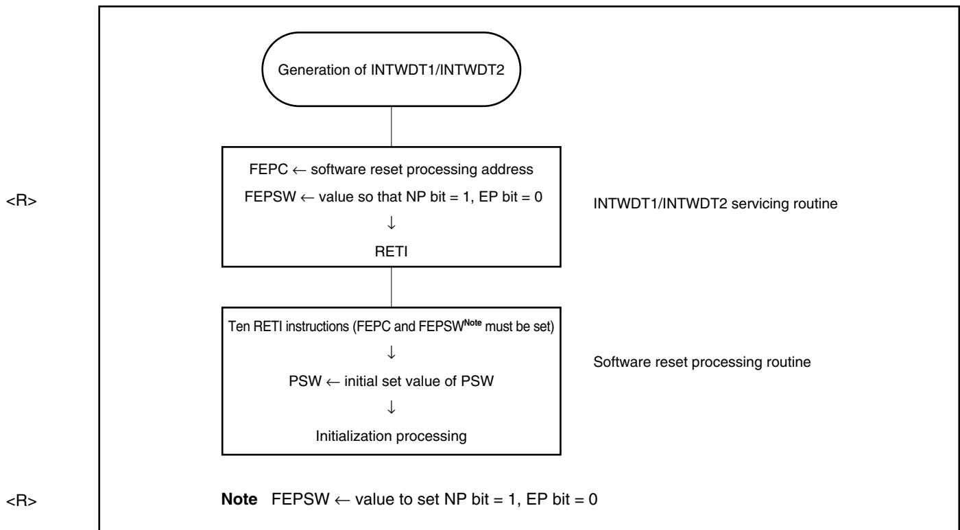
Figure 17-15. Restoring by RETI Instruction
