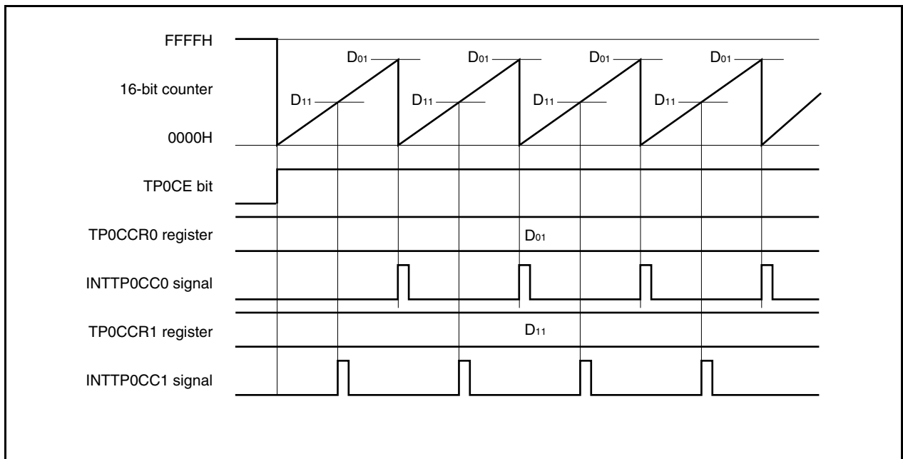
Figure 6-14. Timing Chart When D_{01} \geq D_{11}
