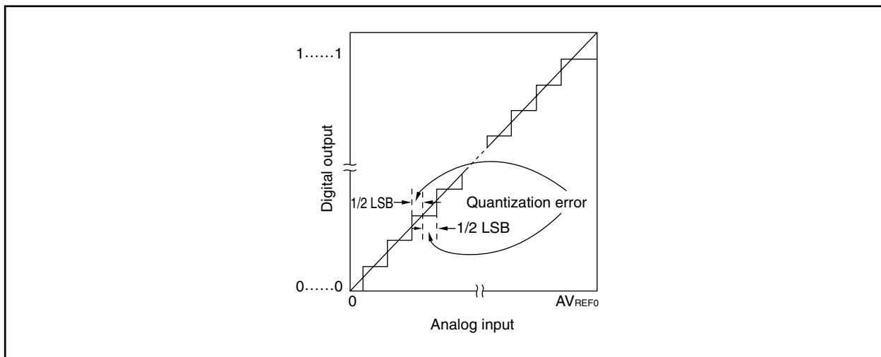
Figure 13-13. Quantization Error
