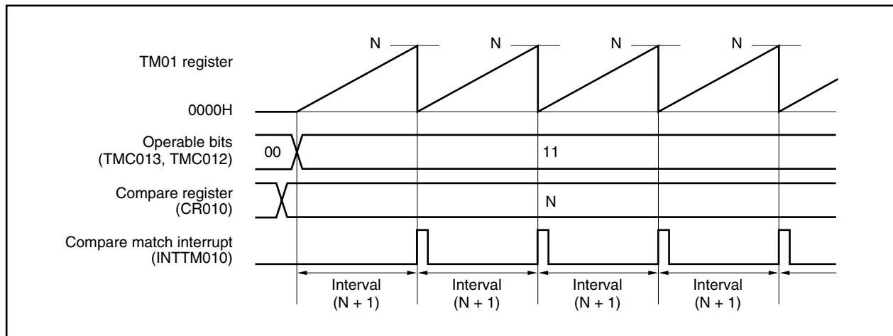
Figure 7-3. Basic Timing Example of Interval Timer Operation
