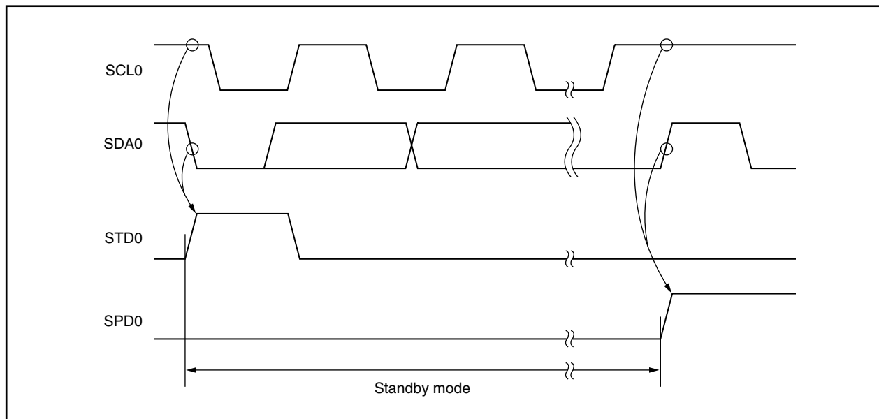
Figure 16-13. Timing for Accepting Communication Reservations
