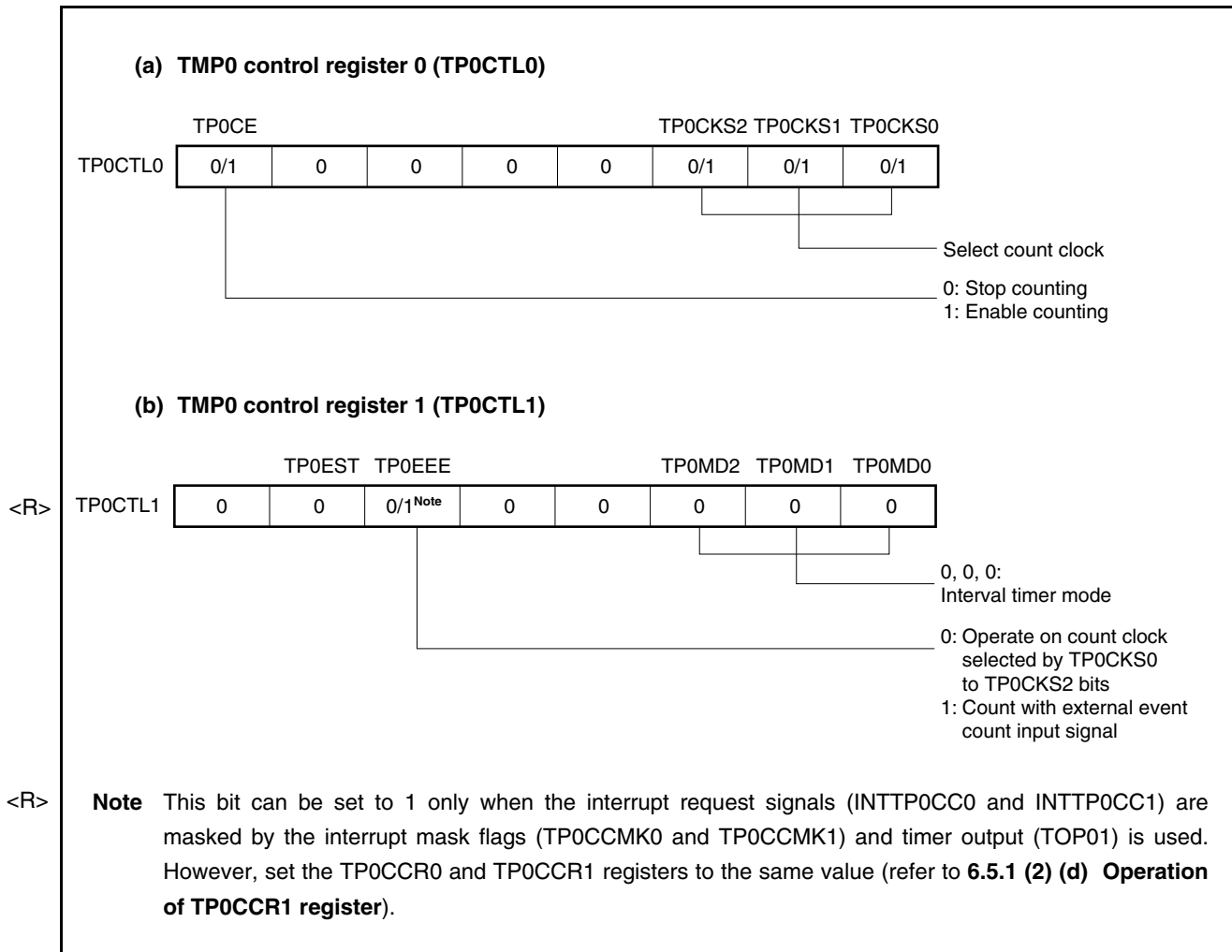
Figure 6-4. Register Setting for Interval Timer Mode Operation (1/2)
