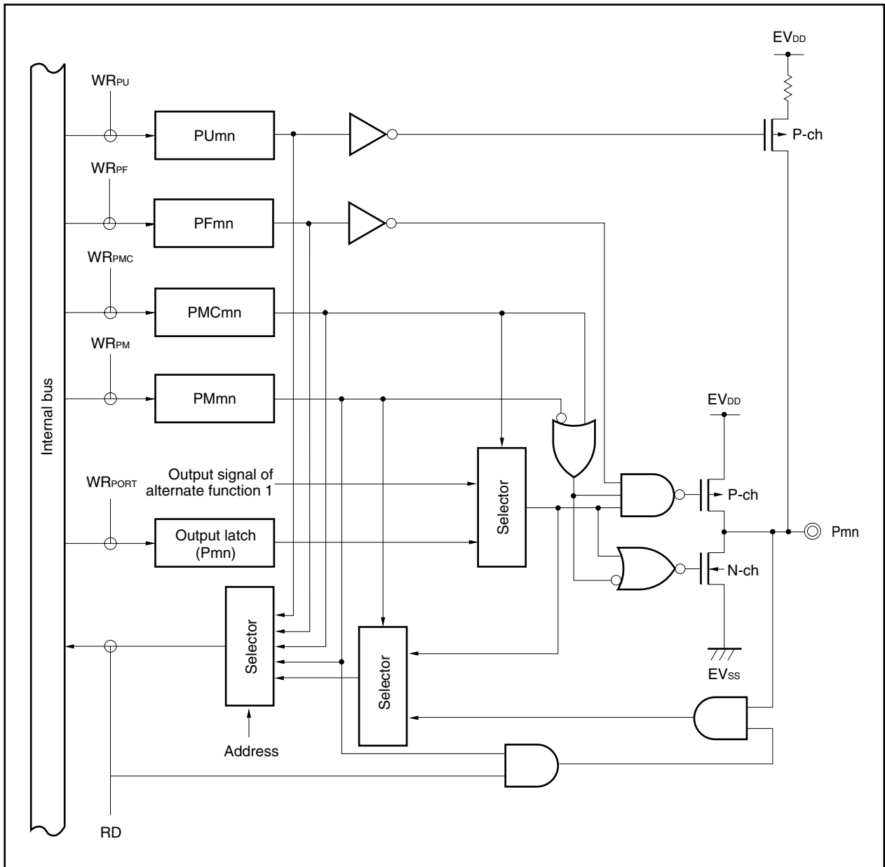
Figure 4-5. Block Diagram of Type D0-UF
