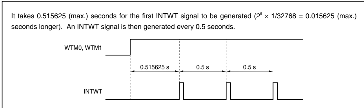
Figure 10-4. Example of Generation of Watch Timer Interrupt Request Signal (INTWT) (When Interrupt Period = 0.5 s)
