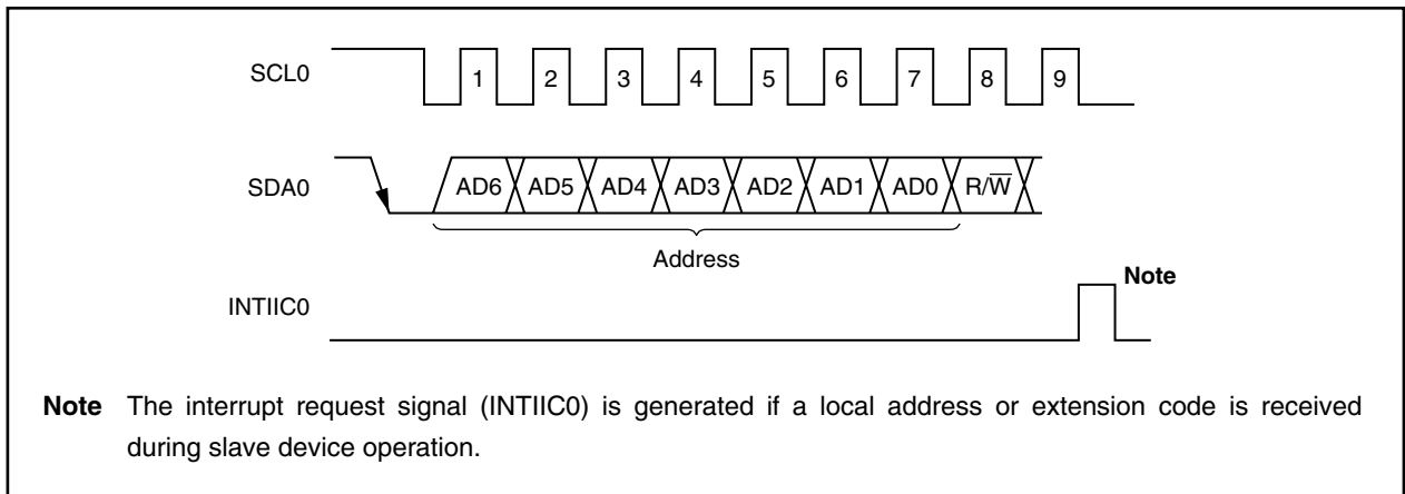
Figure 16-6. Address
