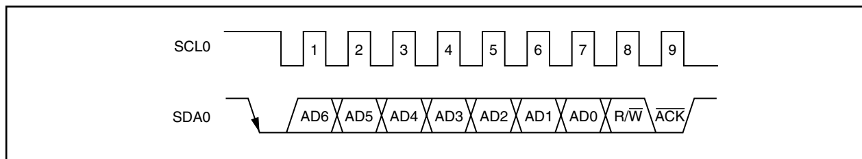
Figure 16-8. \overline{\text{ACK}}
