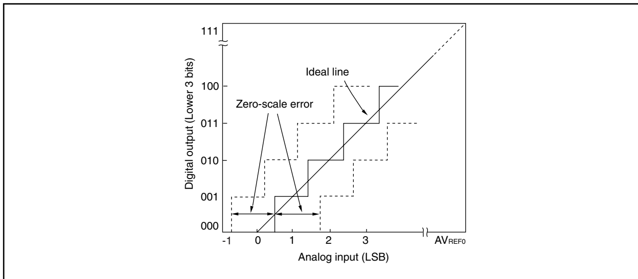
Figure 13-14. Zero-Scale Error
