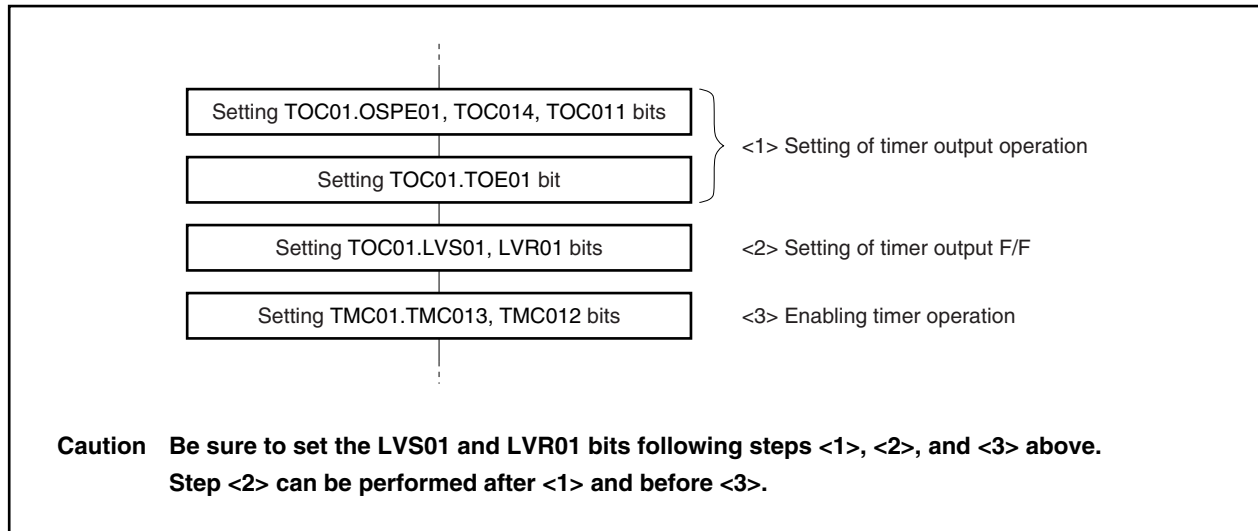
Figure 7-45. Timing Example of LVR01 and LVS01 Bits
