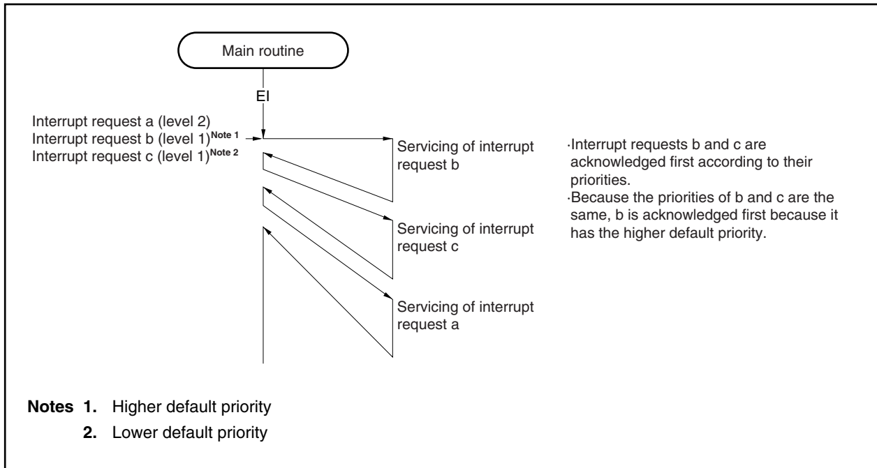
Figure 17-7. Example of Servicing Simultaneously Generated Interrupt Request Signals
