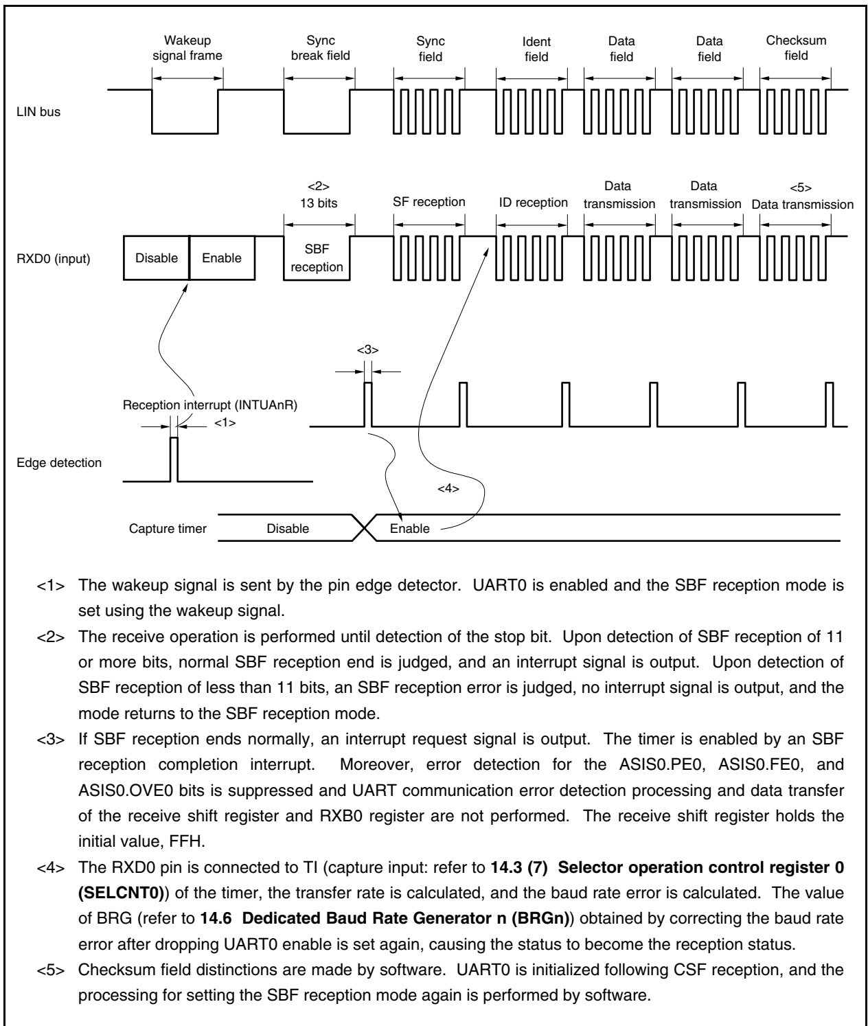
Figure 14-13. LIN Reception Manipulation Outline
