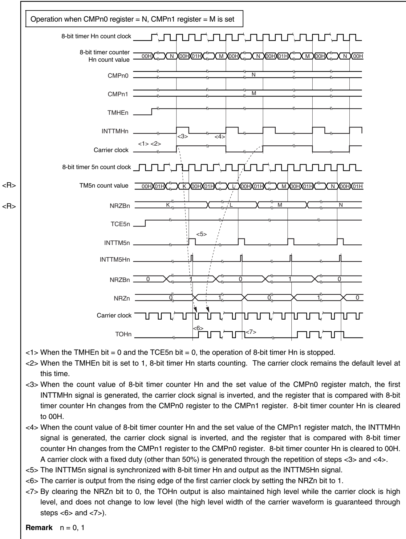
Figure 9-8. Carrier Generator Mode (2/3)
