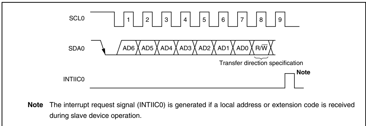
Figure 16-7. Transfer Direction Specification
