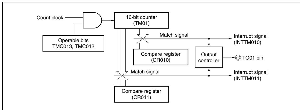
Figure 7-23. Block Diagram of Free-Running Timer Mode (CR010 Register: Compare Register, CR011 Register: Compare Register)
