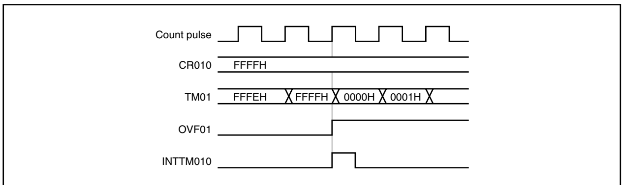
Figure 7-48. Operation Timing of OVF01 Flag
