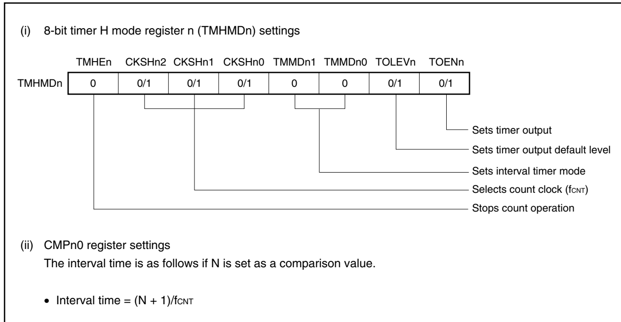
Figure 9-2. Register Settings in Interval Timer Mode
