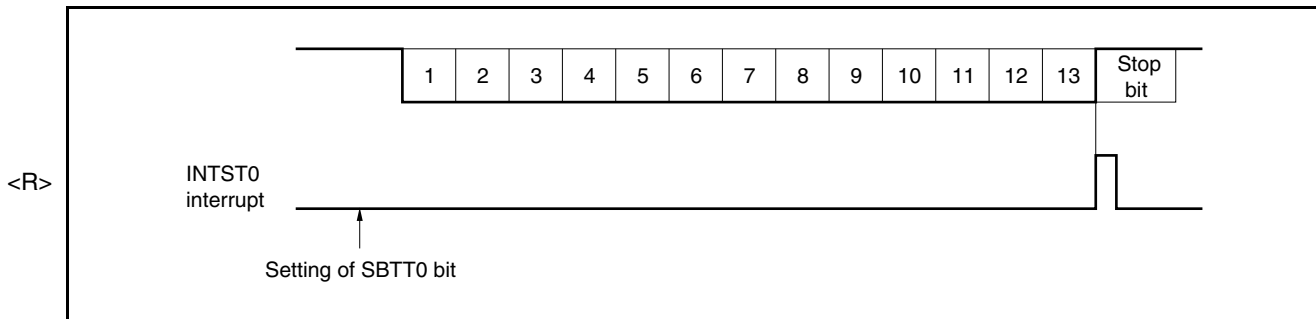
Figure 14-14. SBF Transmission
