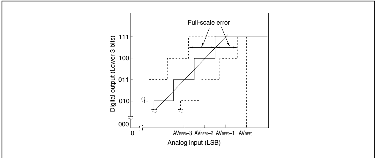
Figure 13-15. Full-Scale Error
