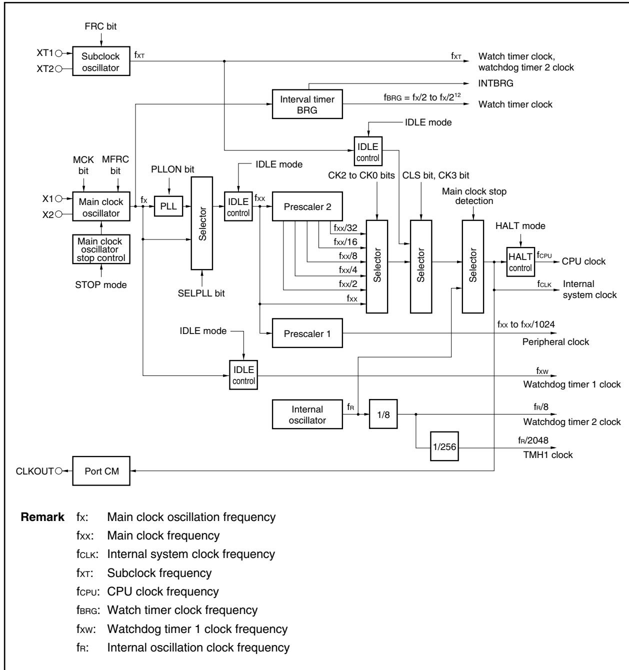
Figure 5-1. Clock Generator
