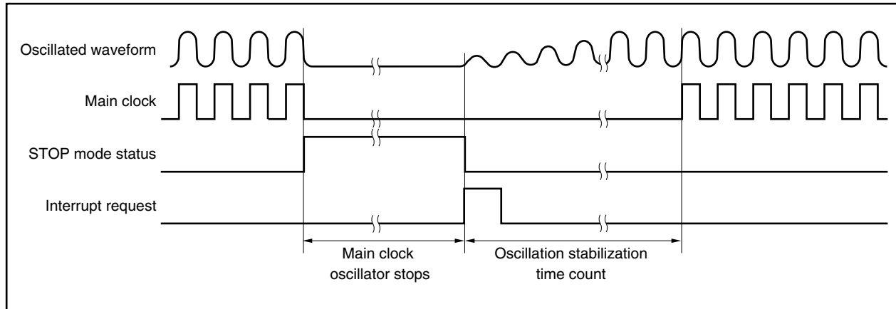
Figure 19-2. Oscillation Stabilization Time
