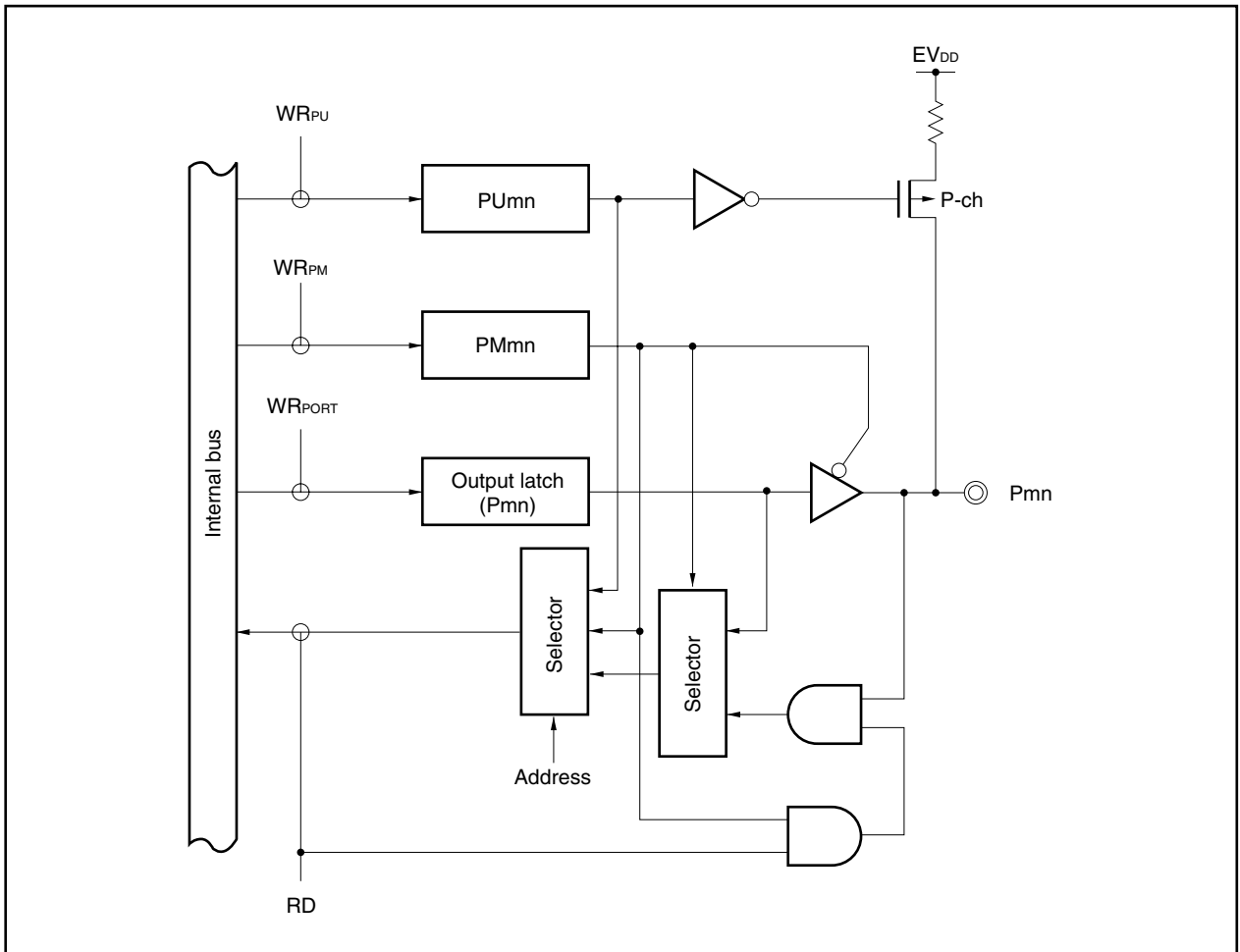
Figure 4-3. Block Diagram of Type C-U
