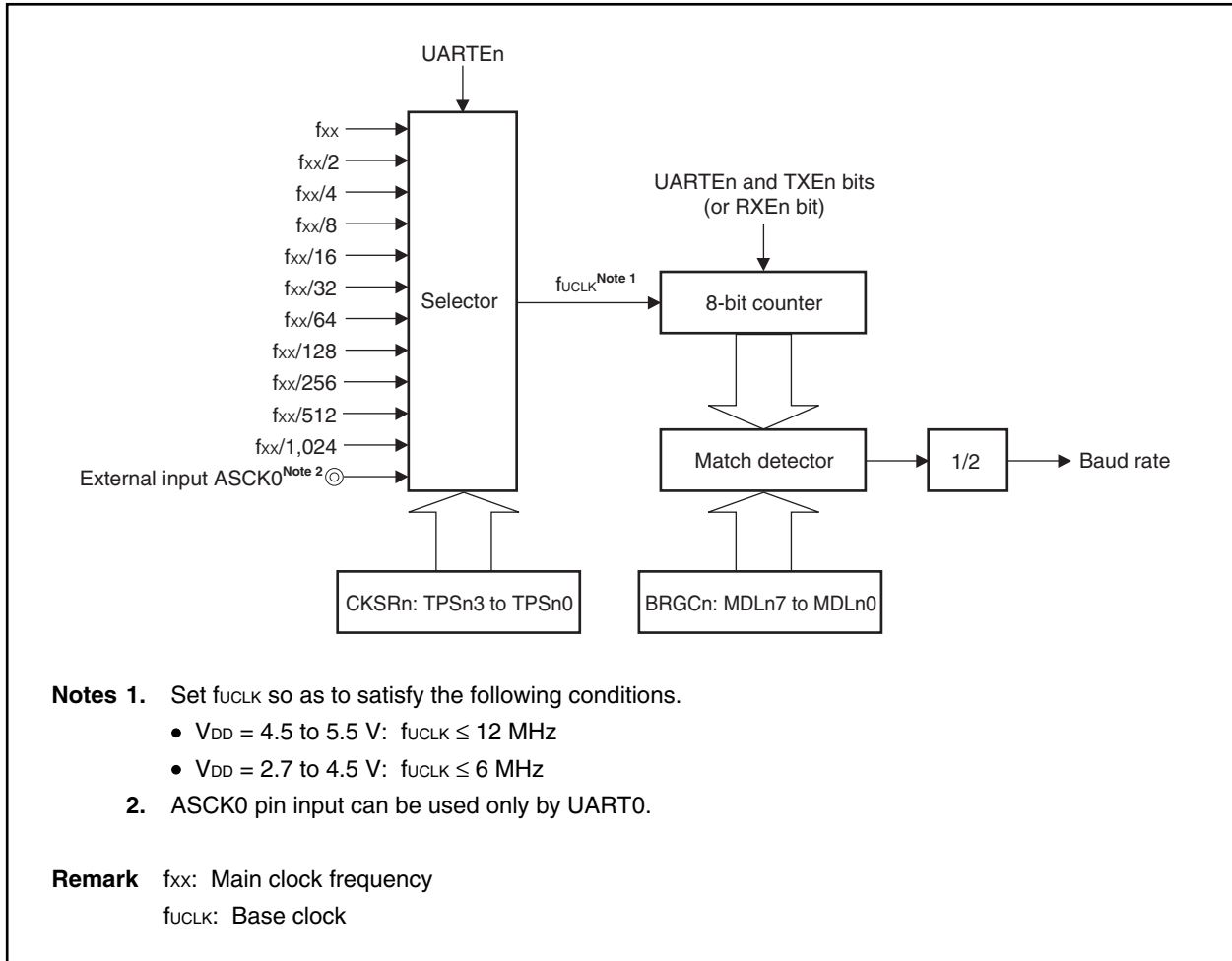
Figure 14-16. Configuration of Baud Rate Generator n (BRGn)
