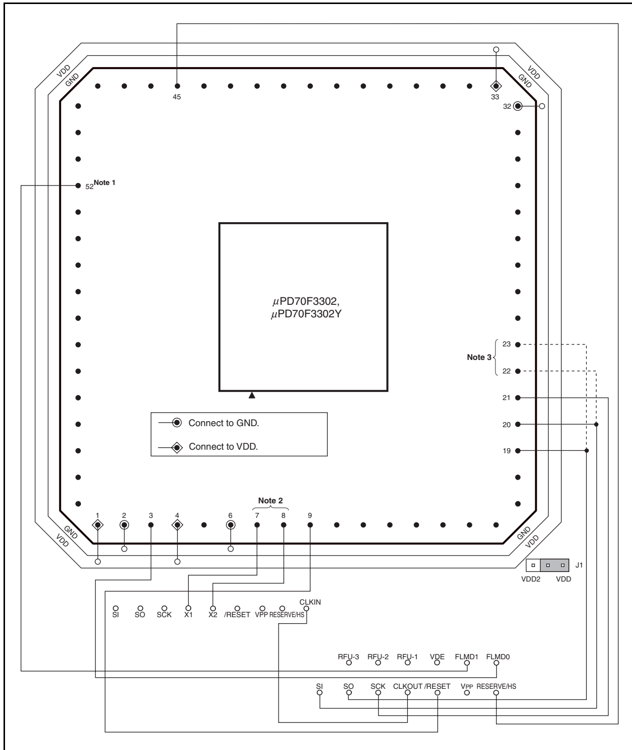
<R> Figure 26-6. Wiring Example of V850ES/KE1+ Flash Writing Adapter (FA-64GK-9ET-A, FA-64GB-8EU-A) (1/2)
