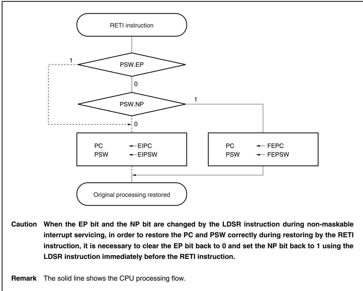
Figure 17-3. RETI Instruction Processing
