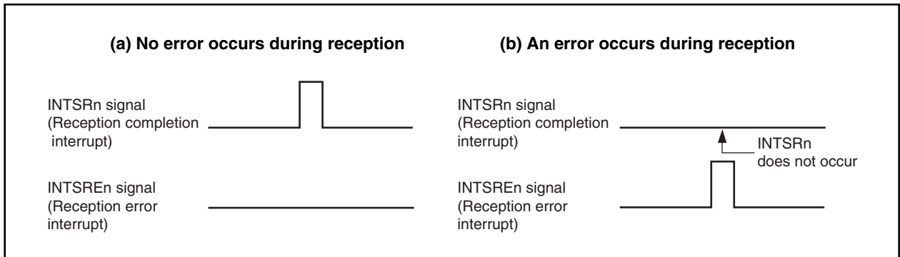
Figure 14-9. When Reception Error Interrupt Request Signal Is Included in INTSRn Signal (ISRMn Bit = 1)
