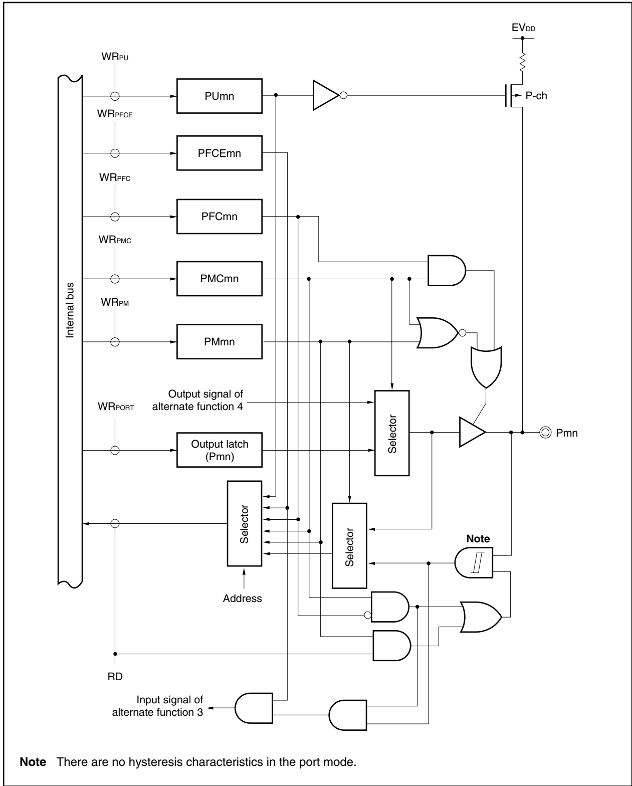
Figure 4-20. Block Diagram of Type Gxx10-SUL
