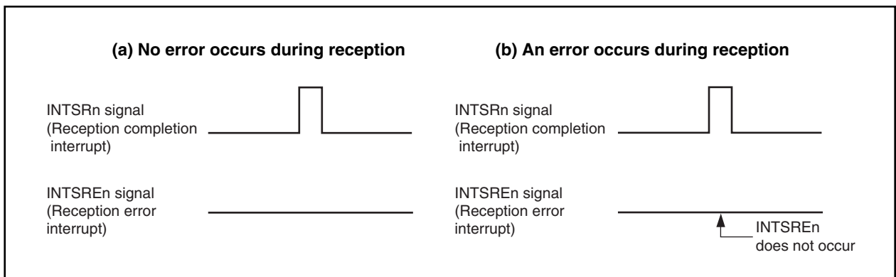
Figure 14-9. When Reception Error Interrupt Request Signal Is Included in INTSRn Signal (ISRMn Bit = 1)
