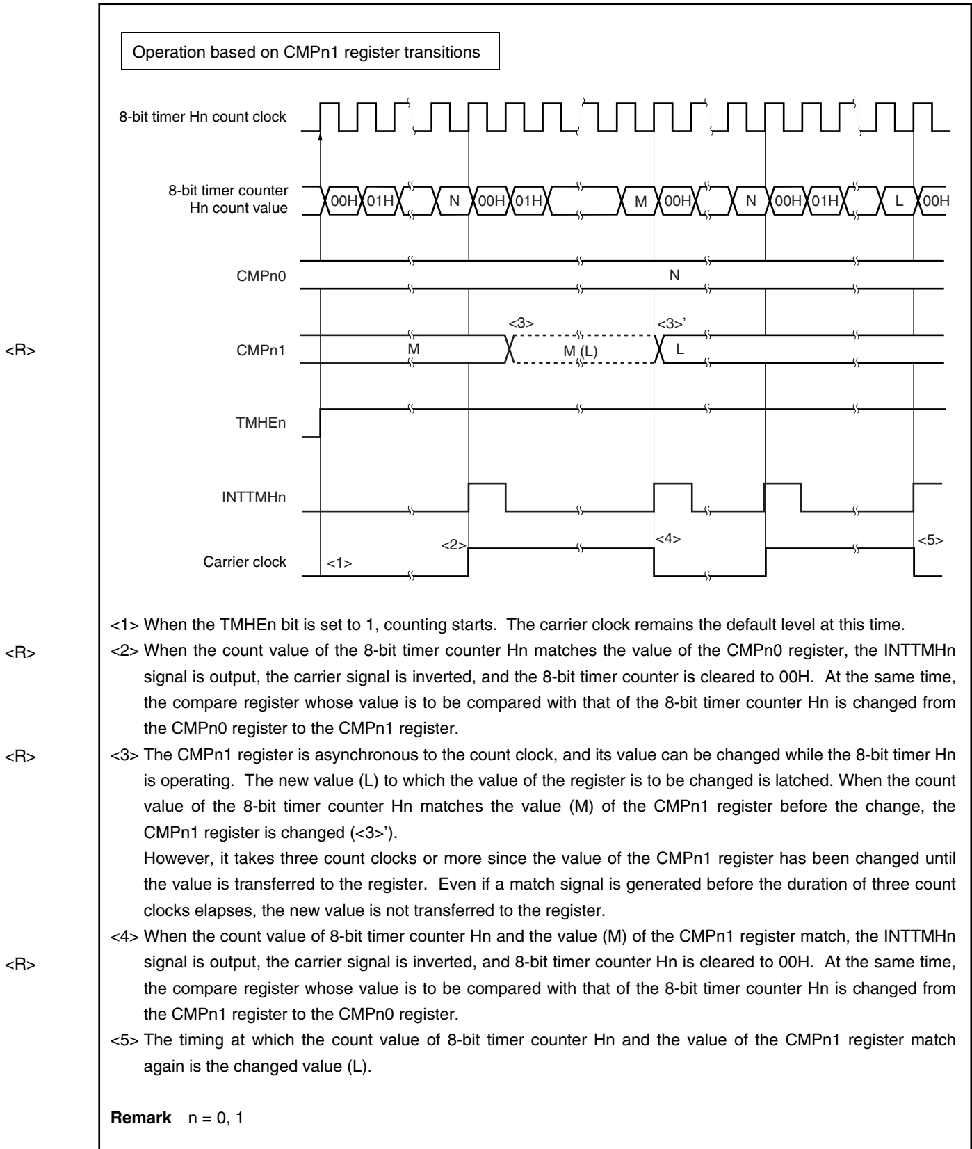
Figure 9-8. Carrier Generator Mode (3/3)
