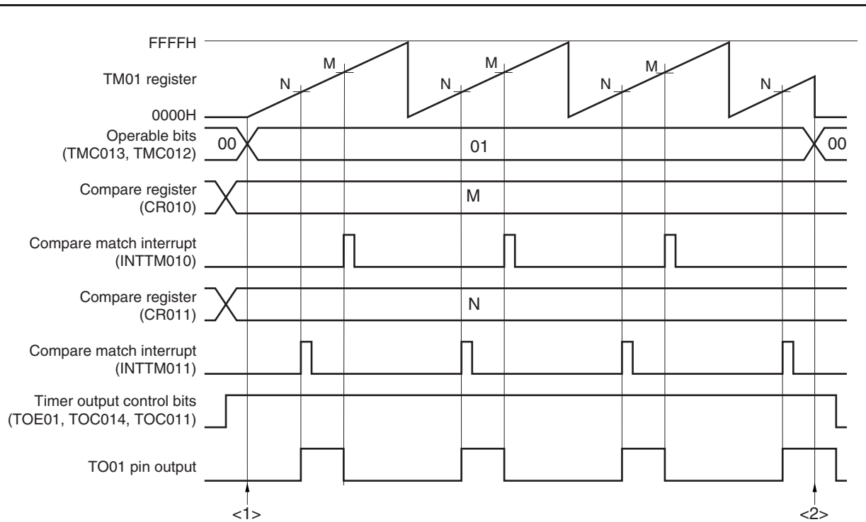
Figure 7-30. Example of Software Processing in Free-Running Timer Mode
