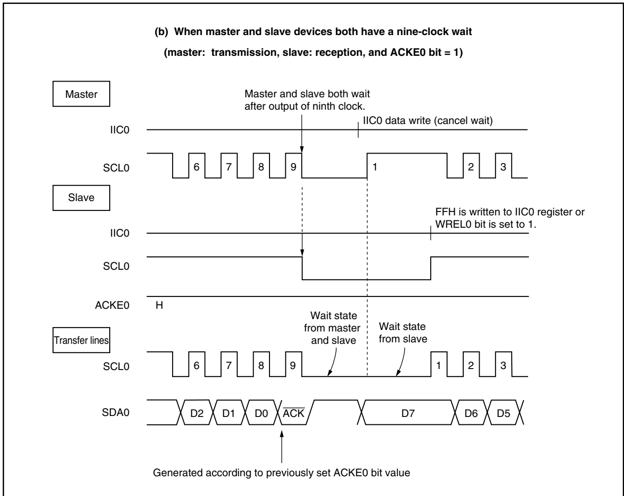
Figure 16-10. Wait State (2/2)
