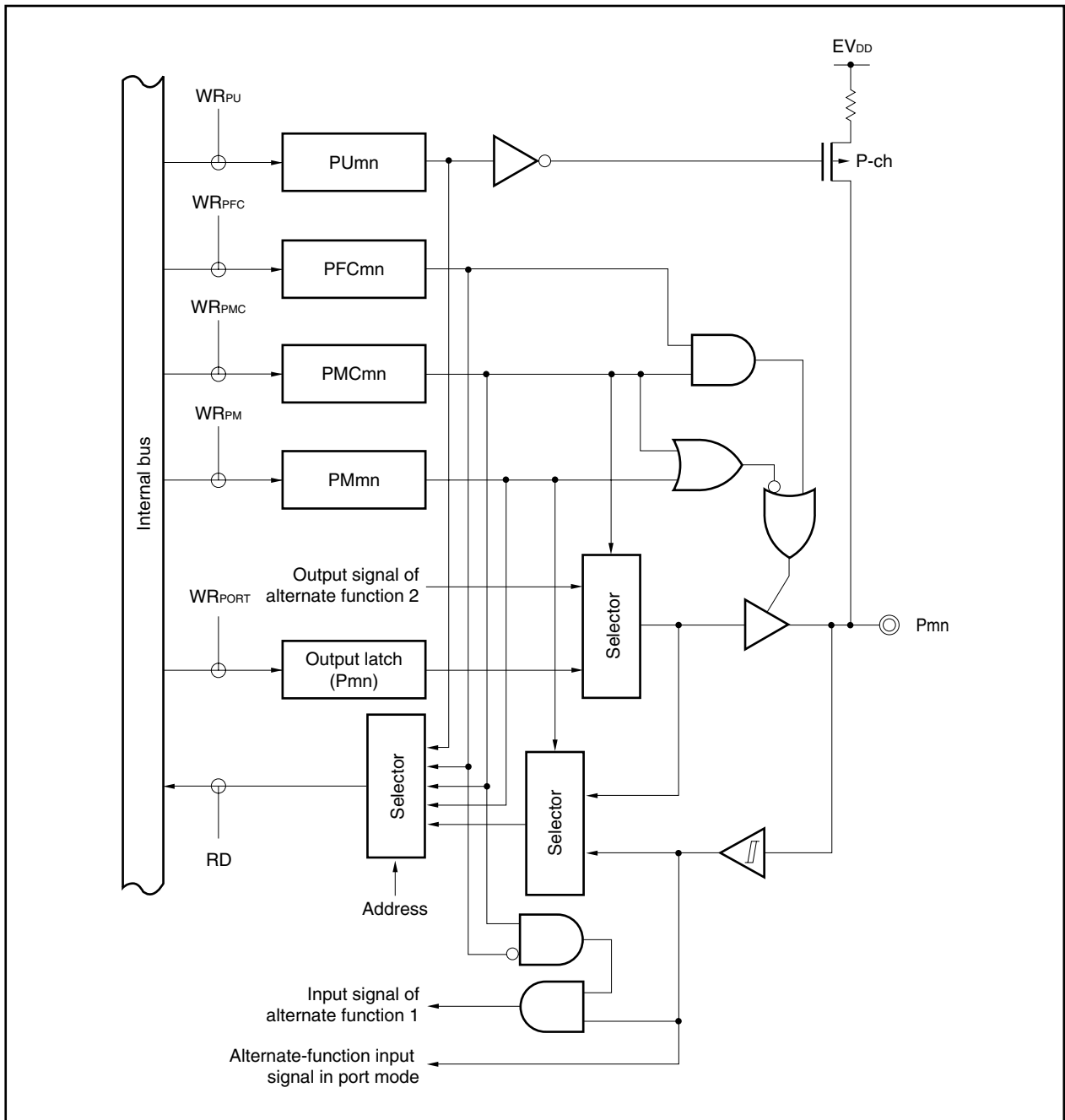
Figure 4-13. Block Diagram of Type E10-SULT
