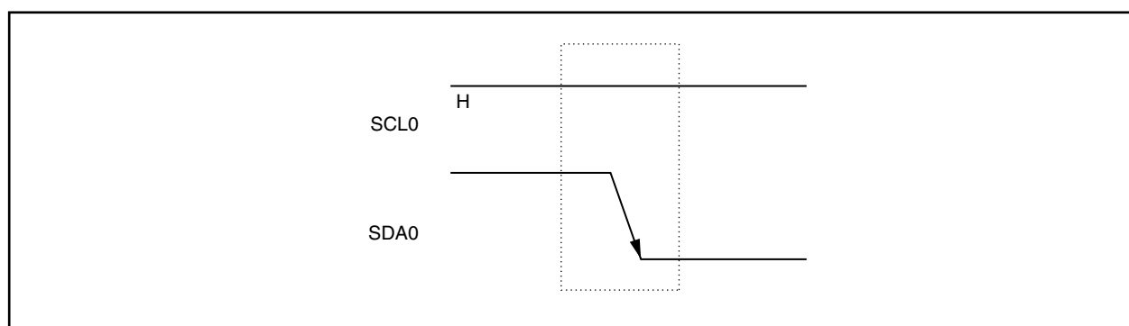
Figure 16-5. Start Conditions
