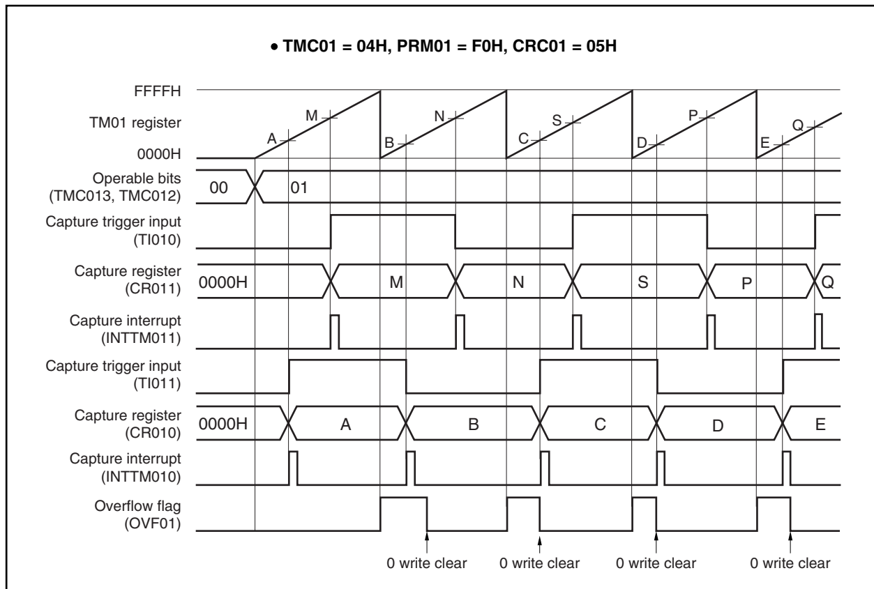
Figure 7-39. Timing Example of Pulse Width Measurement (1)
