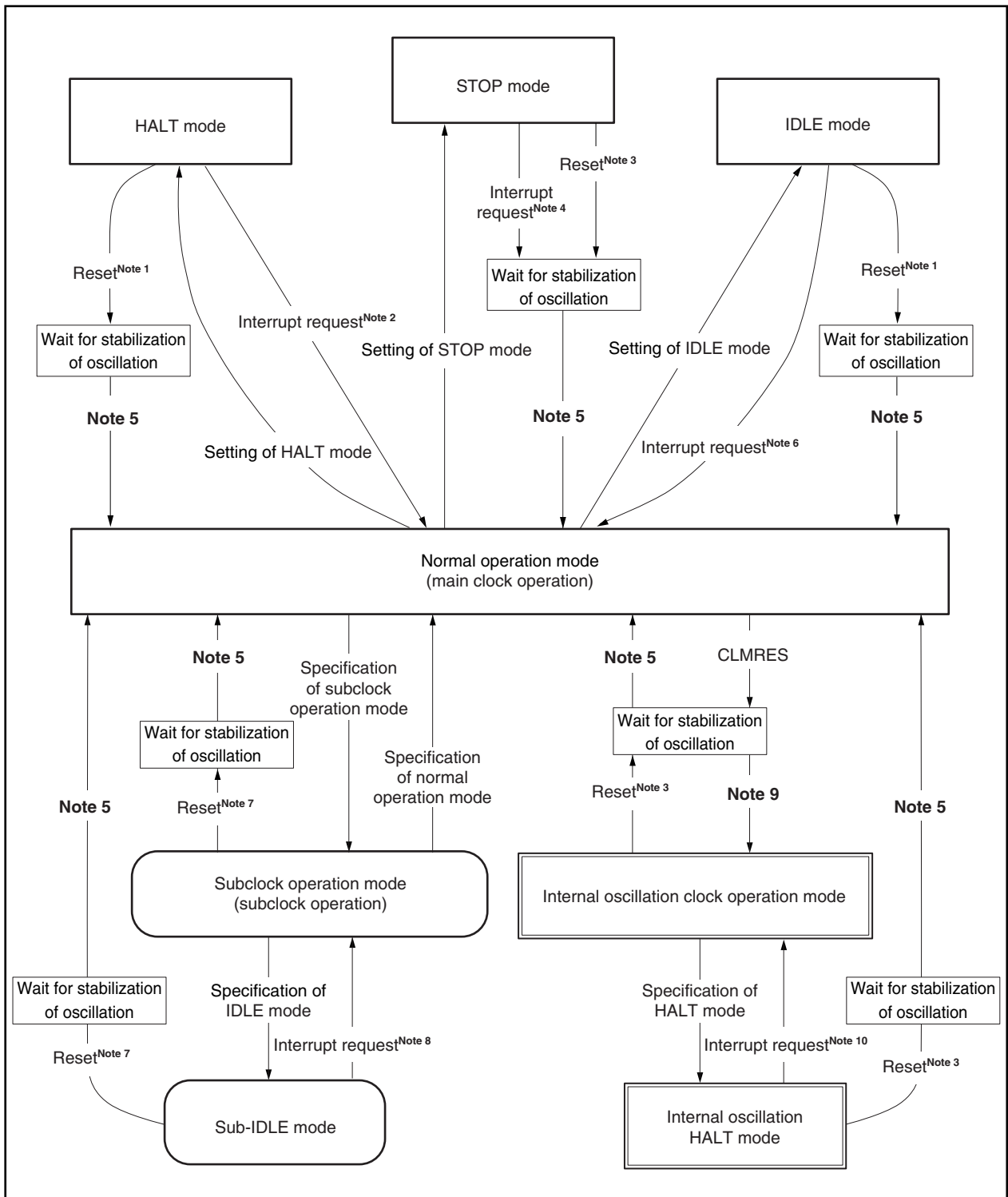
Figure 19-1. Status Transition (1/2)
