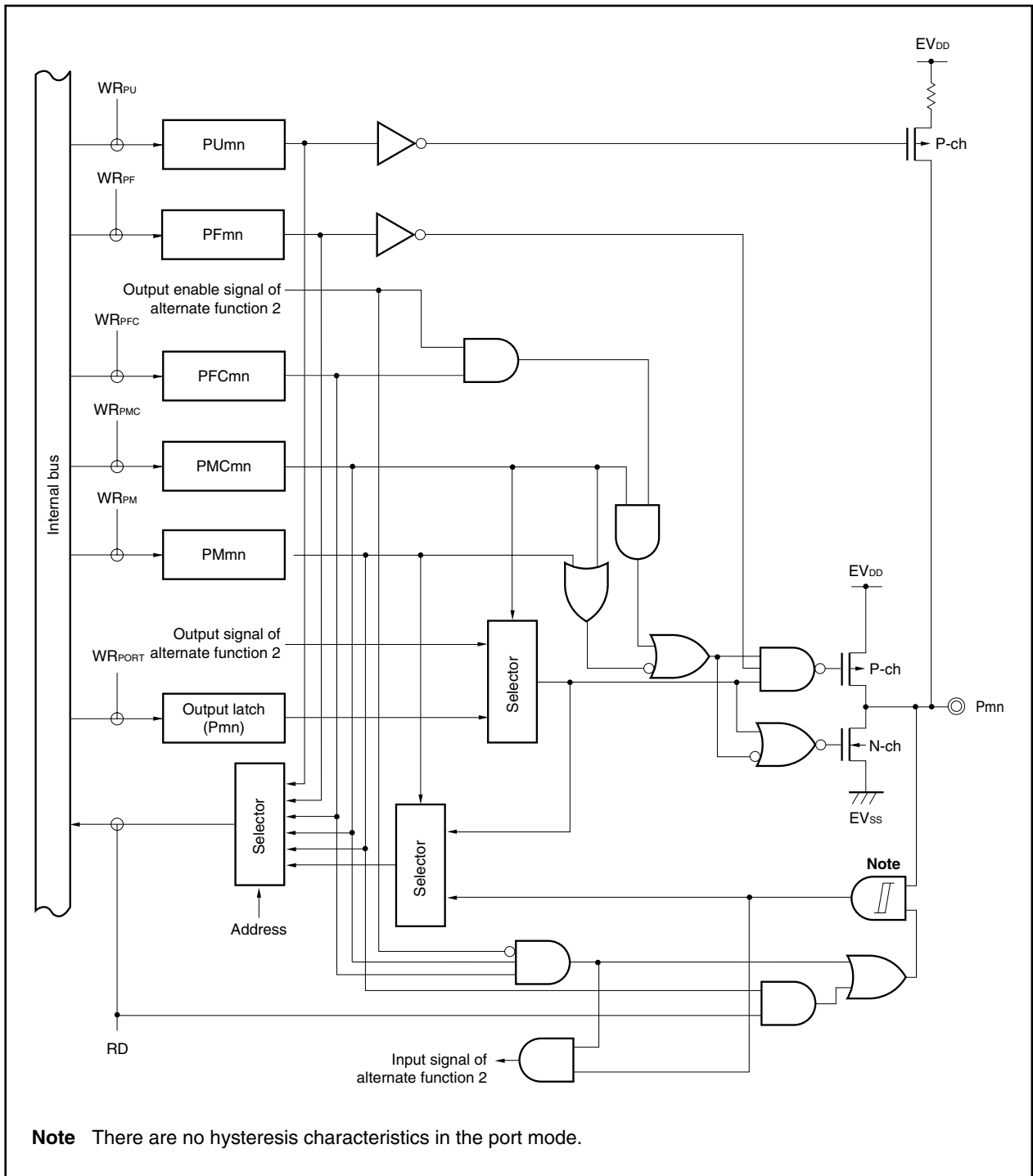
Figure 4-19. Block Diagram of Type Ex2-SUFL
