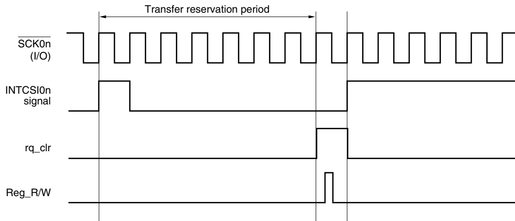
Figure 15-7. Transfer Request Clear and Register Access Conflict
