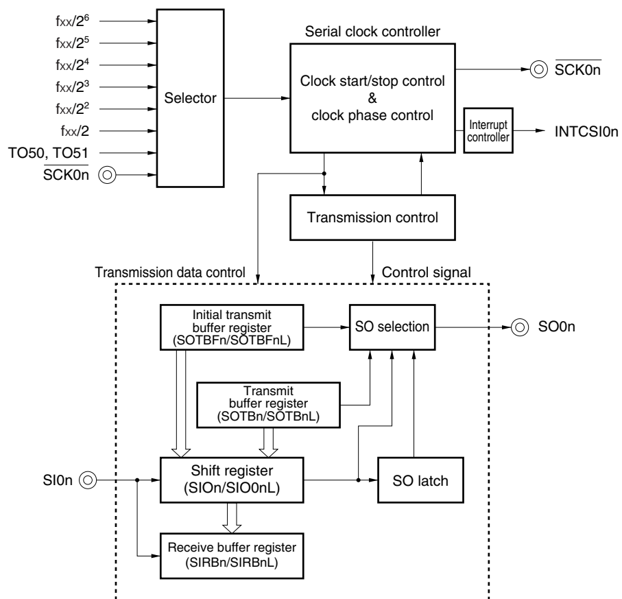
Figure 16-1. Block Diagram of Clocked Serial Interface
