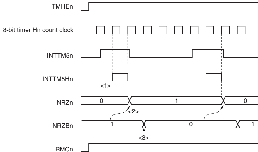
Figure 10-6. Transfer Timing
