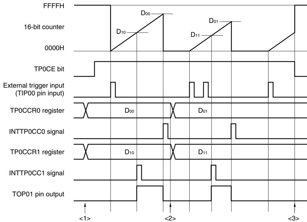
Figure 7-23. Software Processing Flow in One-Shot Pulse Output Mode
