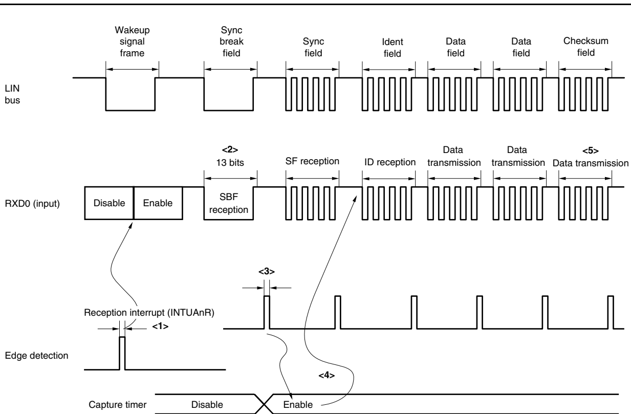
Figure 15-13. LIN Reception Manipulation Outline
