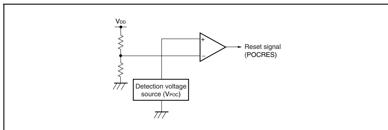
Figure 25-1. Block Diagram of Power-on-Clear Circuit
