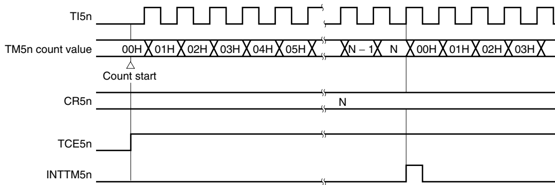
Figure 9-3. Timing of External Event Counter Operation (with Rising Edge Specified)
