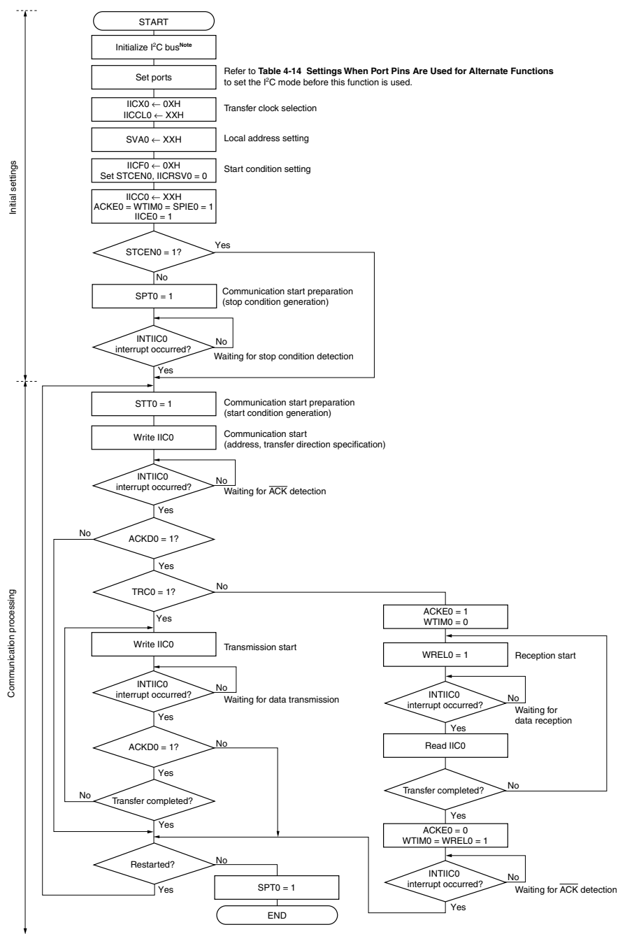
Figure 18-15. Master Operation in Single Master System
