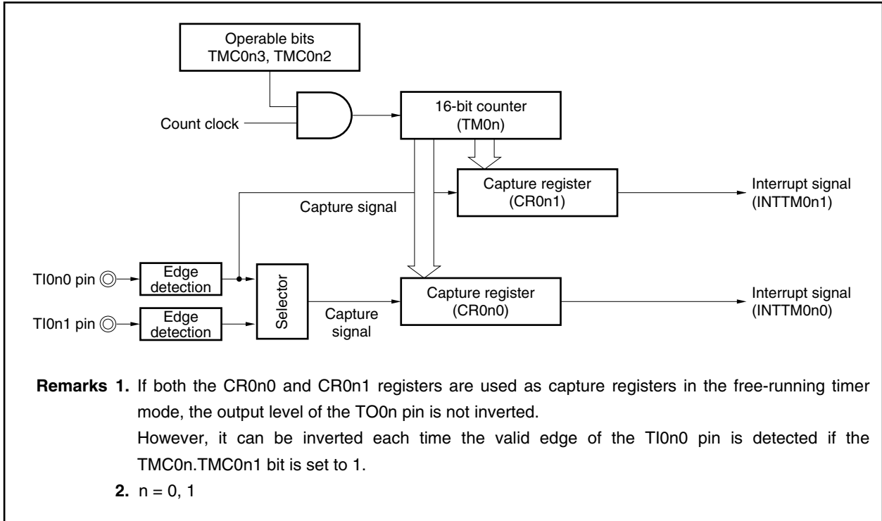
Figure 8-27. Block Diagram of Free-Running Timer Mode
