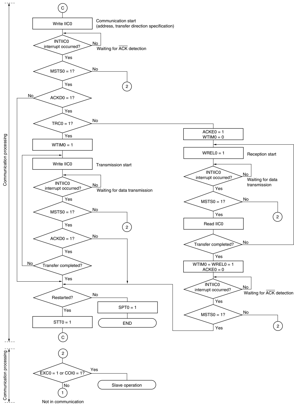
Figure 18-16. Master Operation in Multimaster System (3/3)
