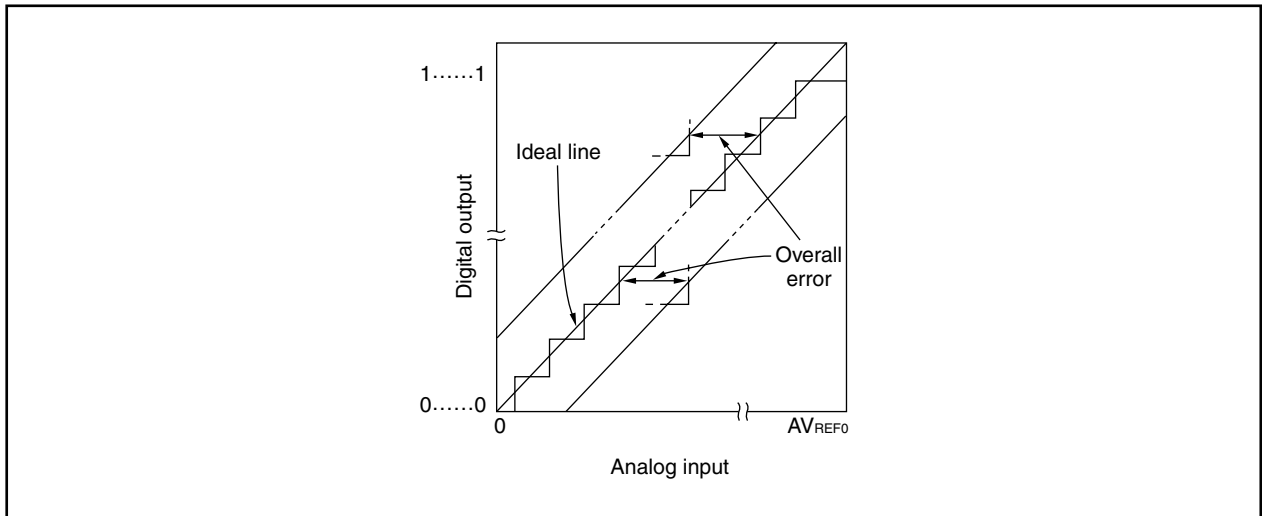
Figure 14-12. Overall Error
