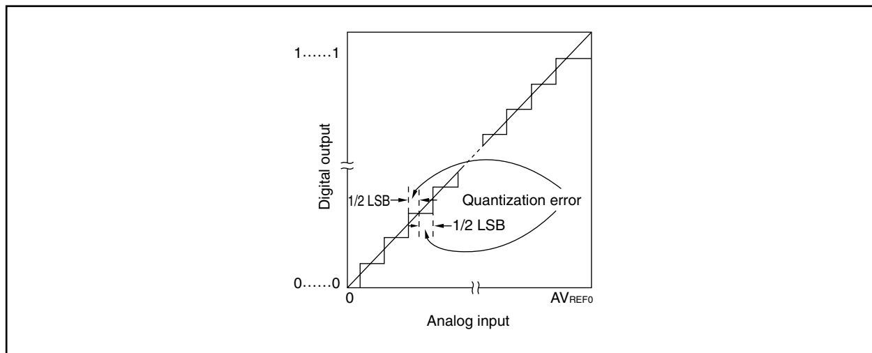
Figure 14-13. Quantization Error
