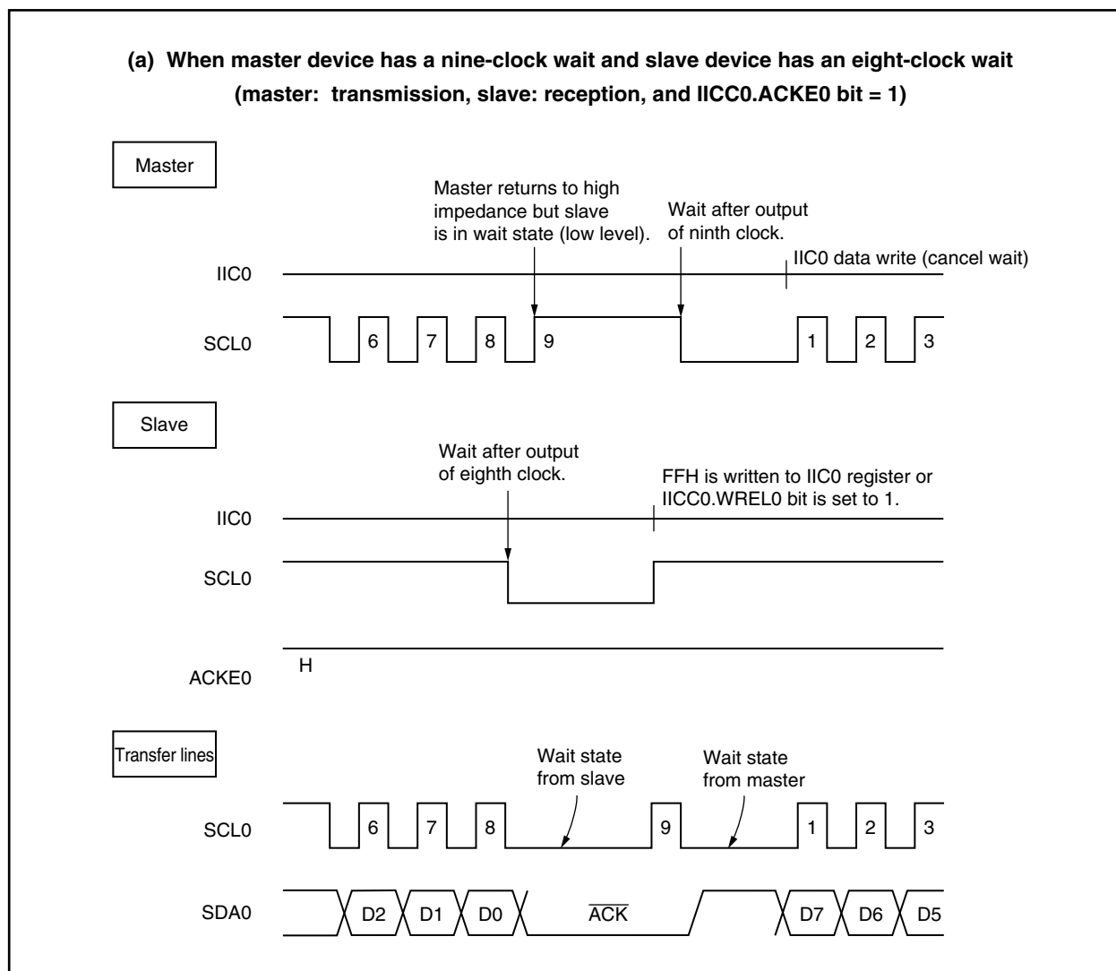
Figure 18-10. Wait State (1/2)
