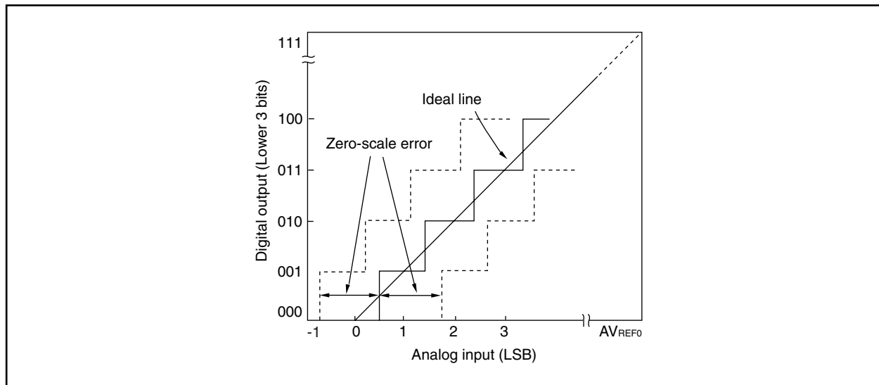
Figure 14-14. Zero-Scale Error
