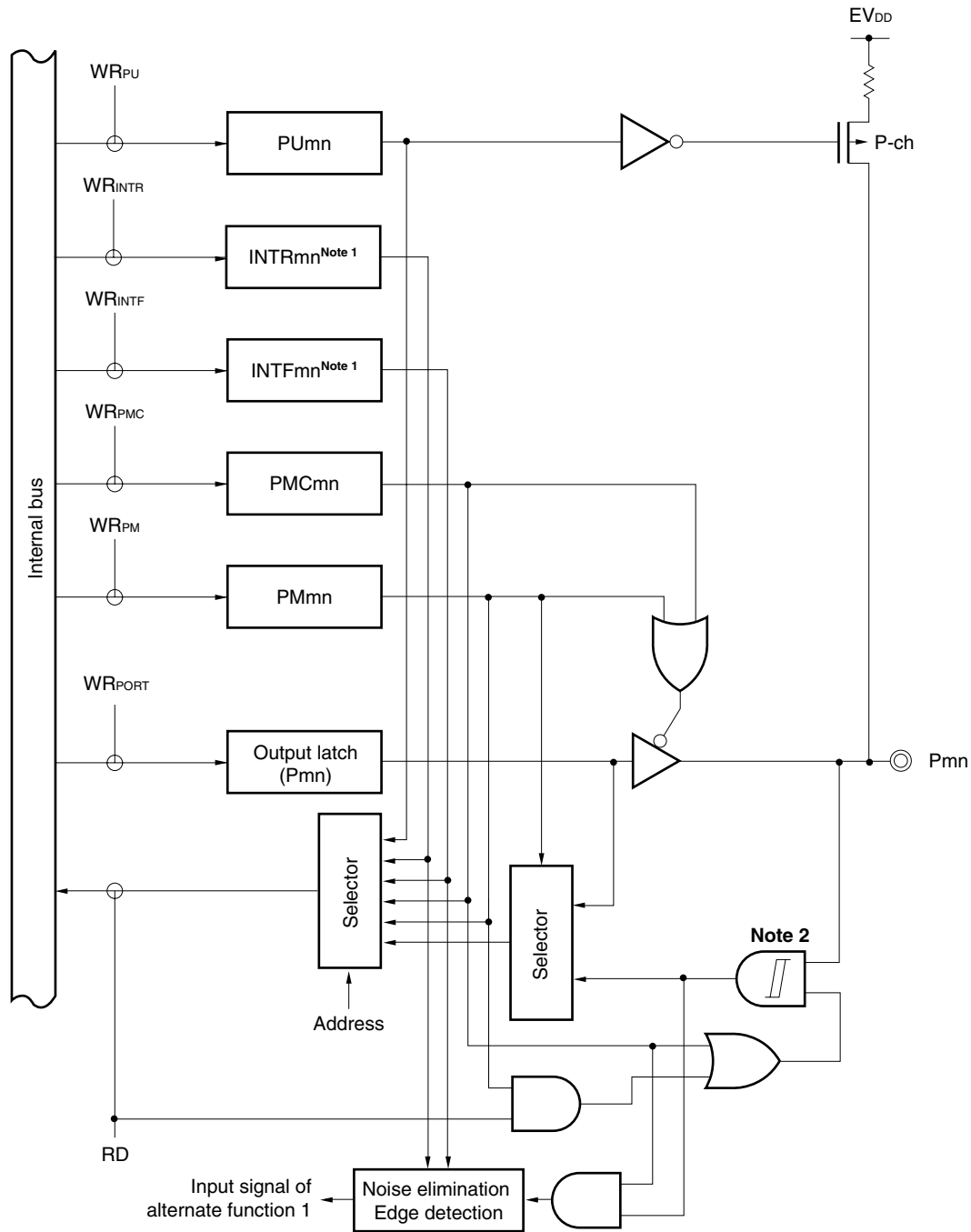
Figure 4-6. Block Diagram of Type D1-SUIL
