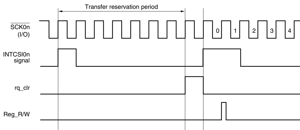
Figure 16-8. Interrupt Request and Register Access Conflict
