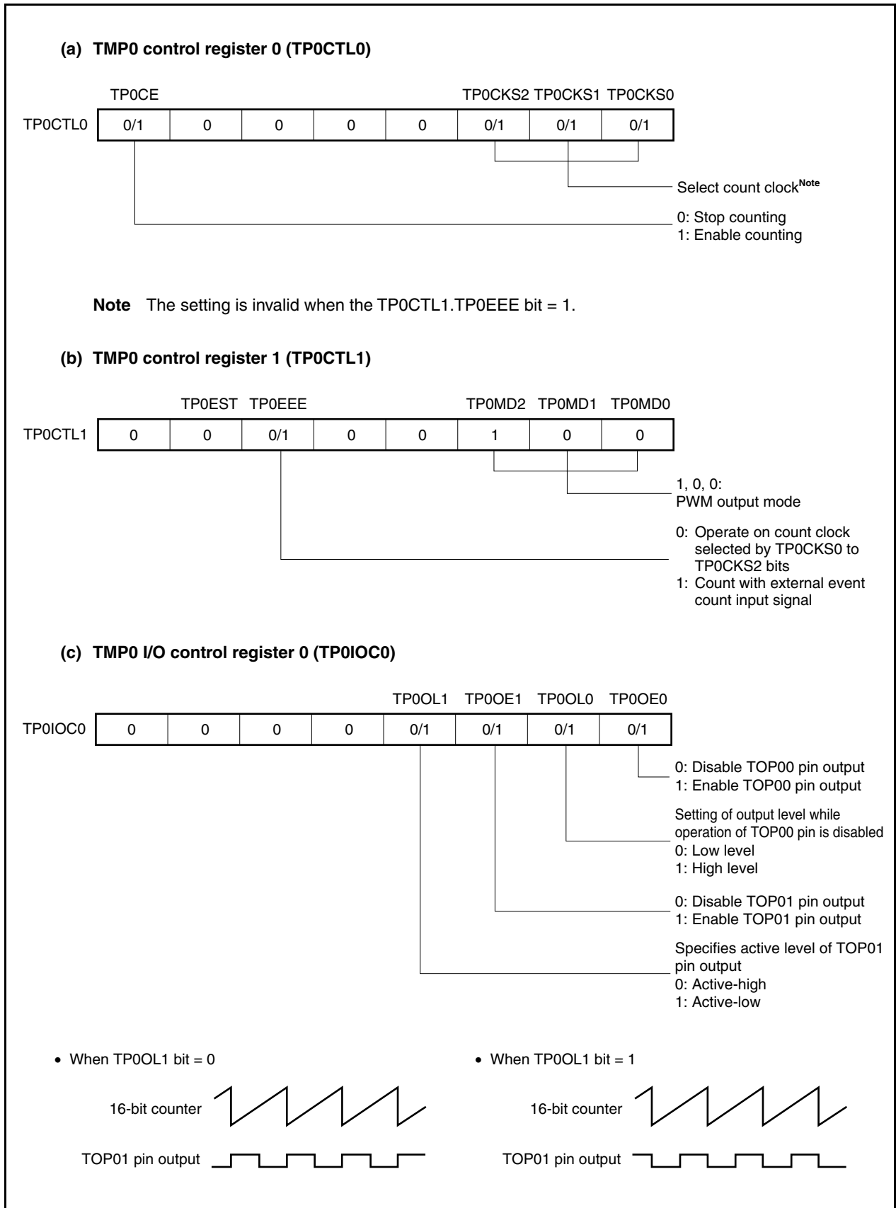
Figure 7-26. Register Setting in PWM Output Mode (1/2)
