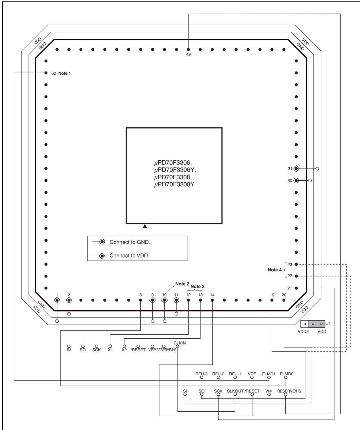
&lt;R&gt; Figure 29-6. Wiring Example of V850ES/KF1+ Flash Writing Adapter (FA-80GC-8BT-A, FA-80GK-9EU-A) (1/2)
