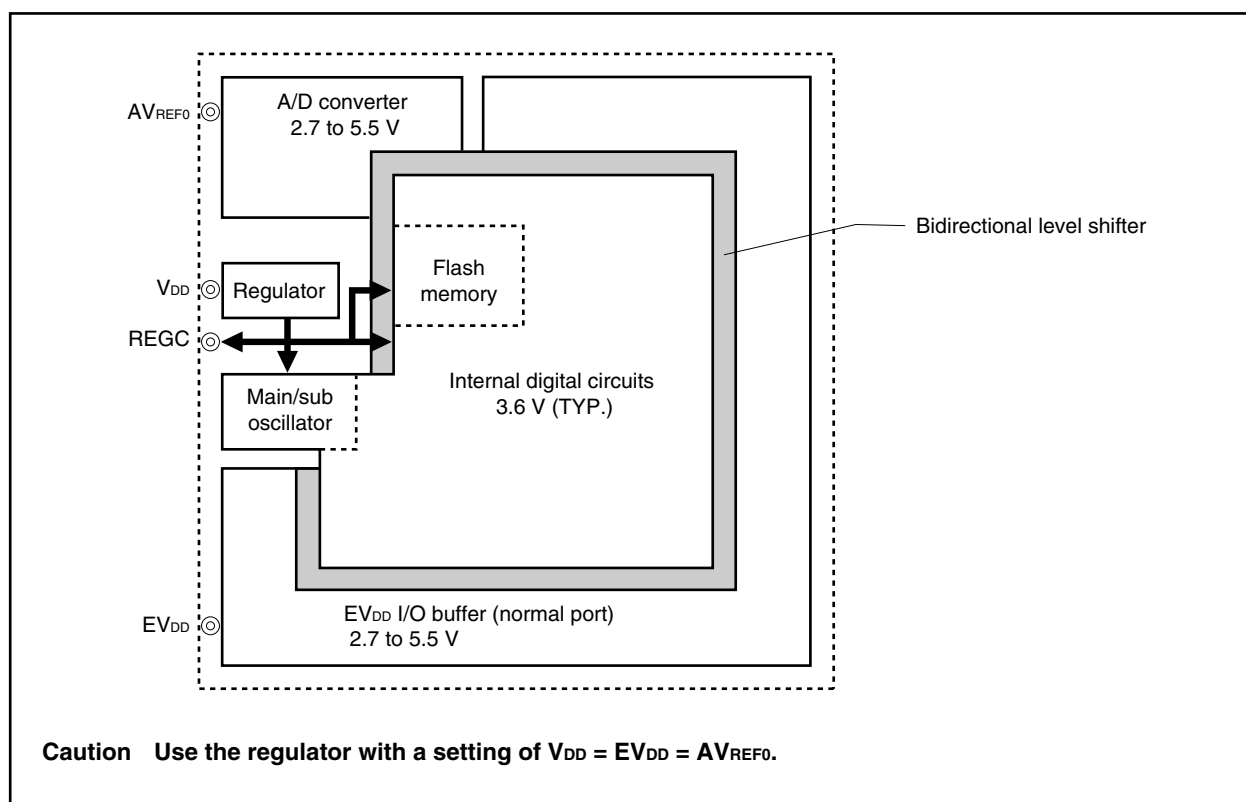
Figure 26-1. Regulator
