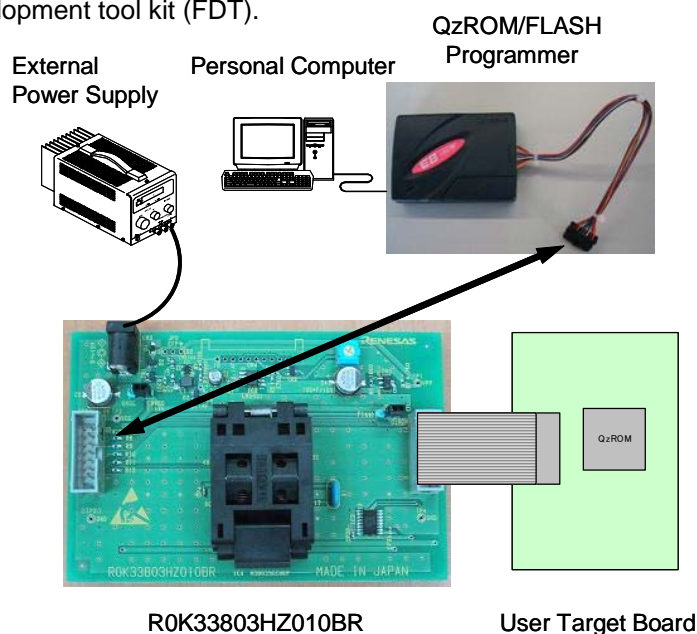
Figure 7.2 Connecting Example 2
