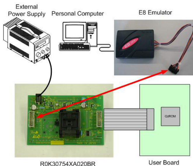
Figure 7.2 Connecting Example 2
