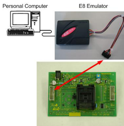
Figure 7.1 Connecting Example 1
