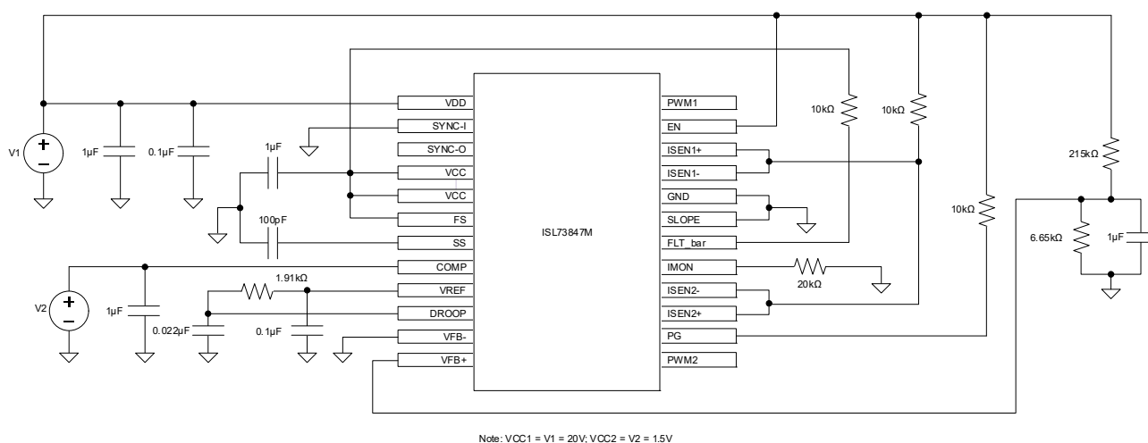
Figure 58. Bias Configuration
