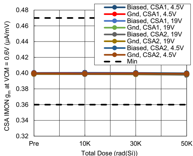
Figure 66. IMON Transconductance vs TID
