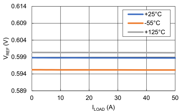
Figure 13. V_{REF} Accuracy for Various Temperatures ( V_{IN} = 5V )
