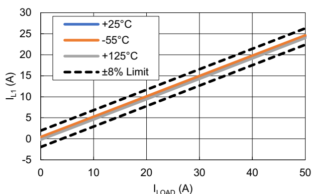
Figure 15. Phase 1 Current Share vs Temperature ( V_{IN} = 5V )
