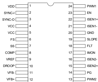
Figure 6. Pin Assignments - 24 Ld SOIC Top View
