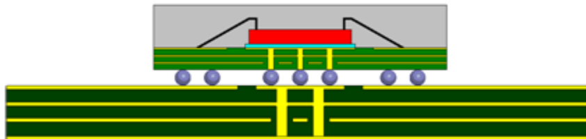
Figure 17. 324 ball, 19mm x 19mm BGA with 4-Layer Substrate
