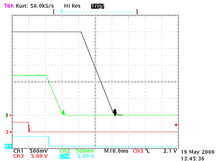
Figure 3. Disable Sequence
