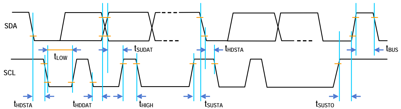
Figure 14. Timing Diagram
