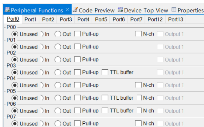
Figure 3-1 Code Generator view
