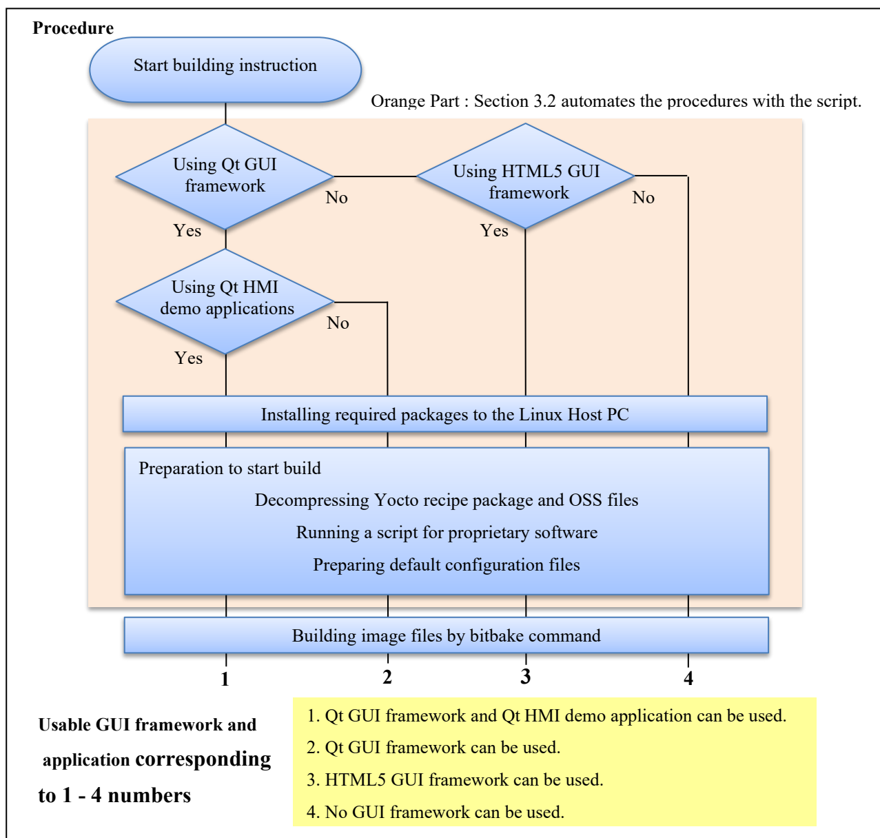
Figure 2. Building Outline
